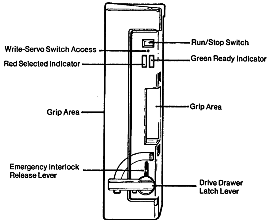
Figure 3-2. Removable Disk Cartridge Controls and Indicators
