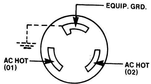
NEMA L6-20P 208/230V, 20A, 60HZ 2 POLE, 3 WIRE, LOCKING CONN.
