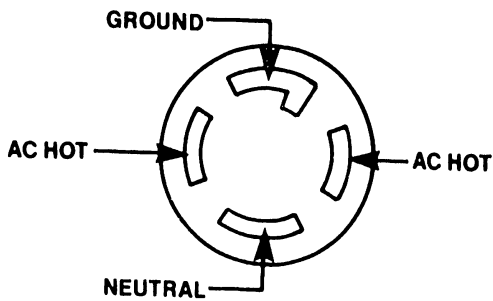
NEMA L14-30R & P HUBBEL 2711 & 10 250V, 30A, 50Hz SPLIT PHASE, 3 POLE 4 WIRE, TWISTLOCK.
