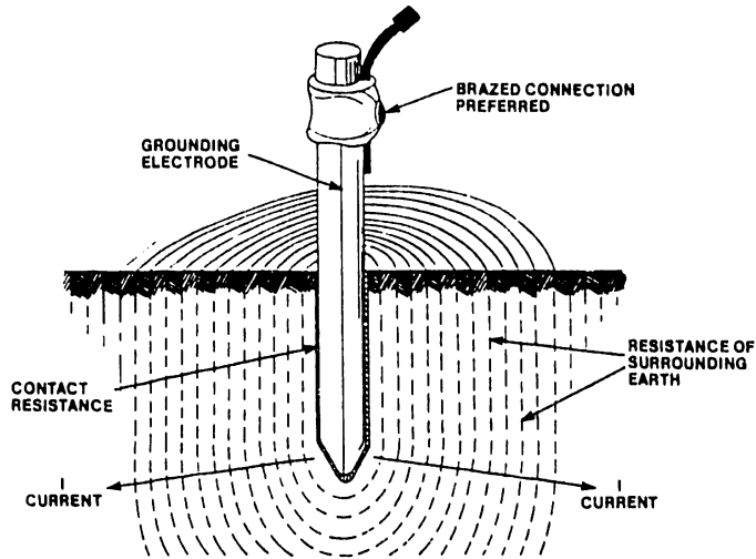
FIGURE 4-5 EARTH GROUND STAKE (Ground Rod)
