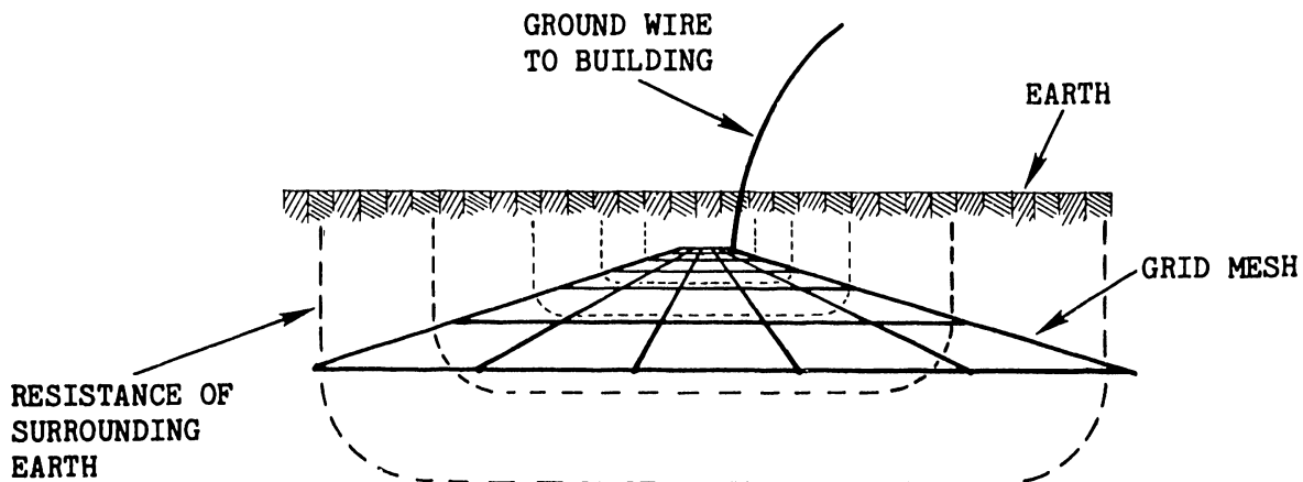
FIGURE 4-6 EARTH GROUND GRID MESH
