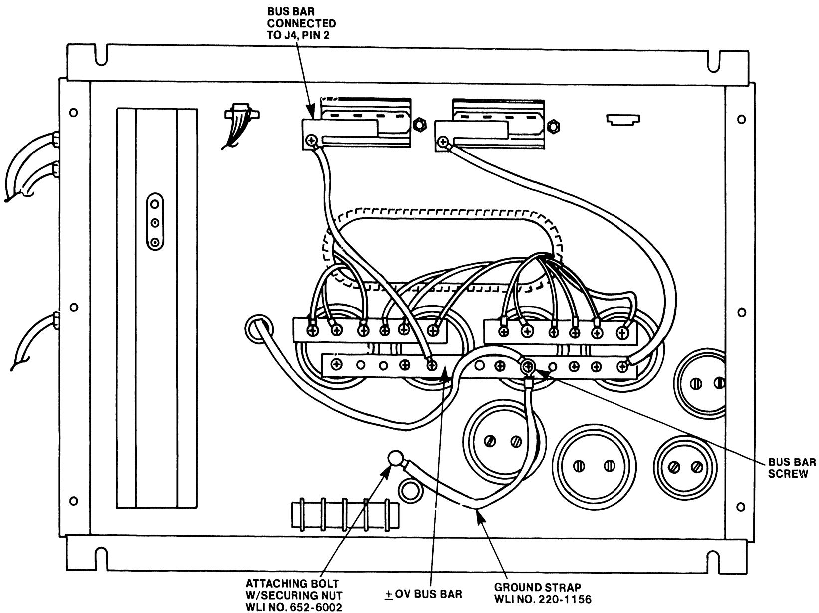
FIGURE 5-1 VS 60/80 POWER SUPPLY (Bottom View)
