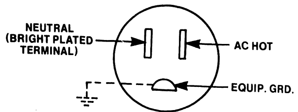
NEMA 5-15G 120V, 15A, 60Hz, SGL PHASE, 2-POLE 3 WIRE.
