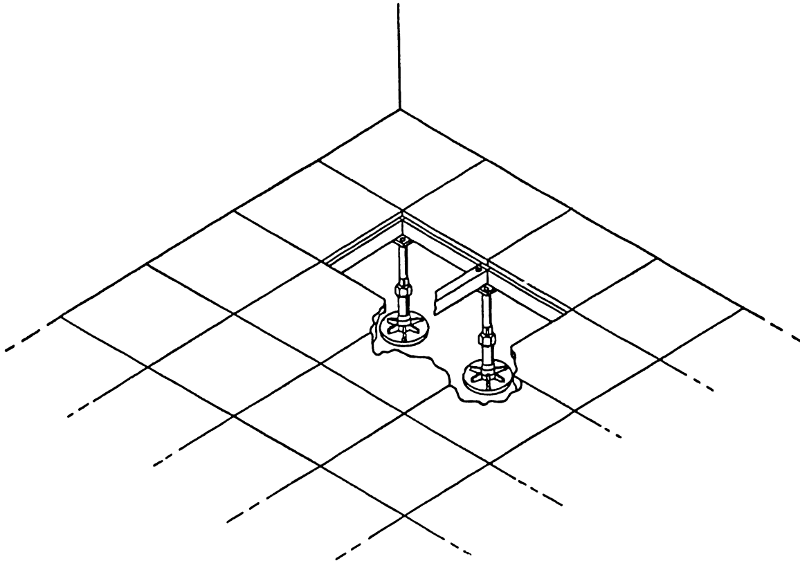
FIGURE 2-2 PEDESTAL-TYPE RAISED FLOORING
