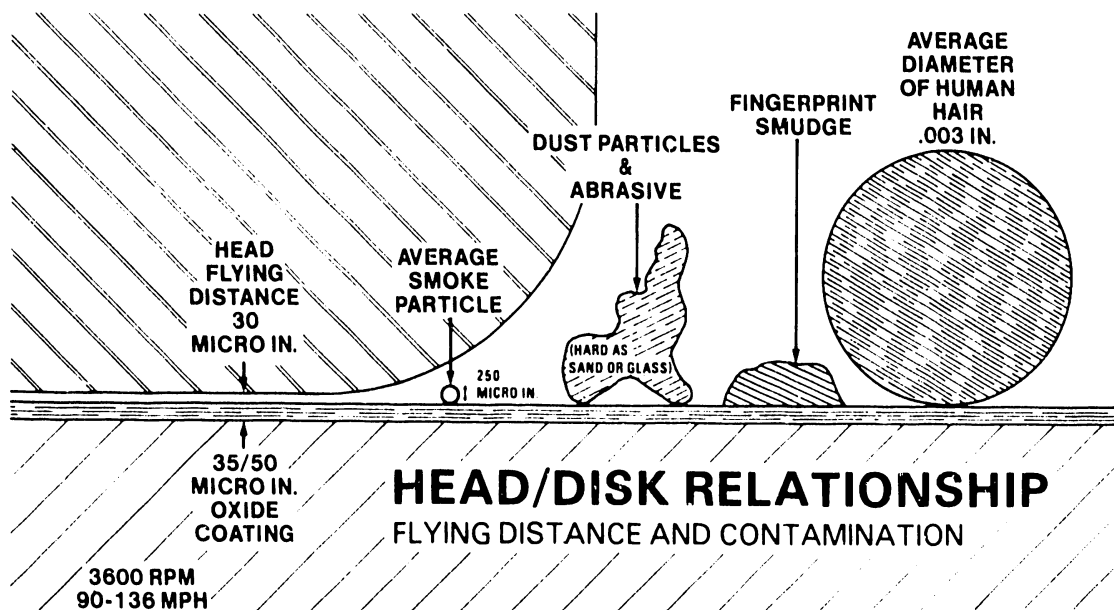
FIGURE 3-1 HEAD/DISK GAP IN RELATION TO POSSIBLE CONTAMINANTS
