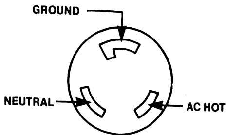
NEMA L5-30P & R HUBBEL NO. 2611 & 10 120V, 30A SGL PHASE
