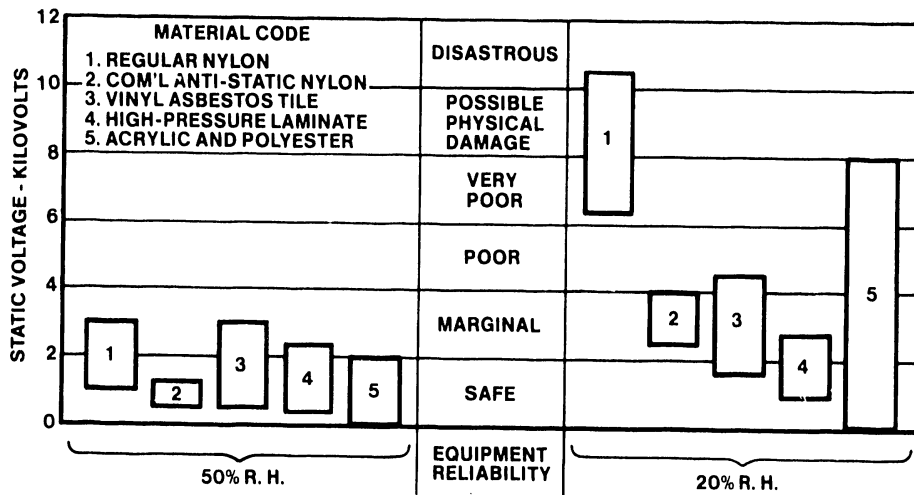
TYPICAL STATIC VOLTAGES GENERATED BY WALKING ON COMMON FLOOR COVERING MATERIALS
