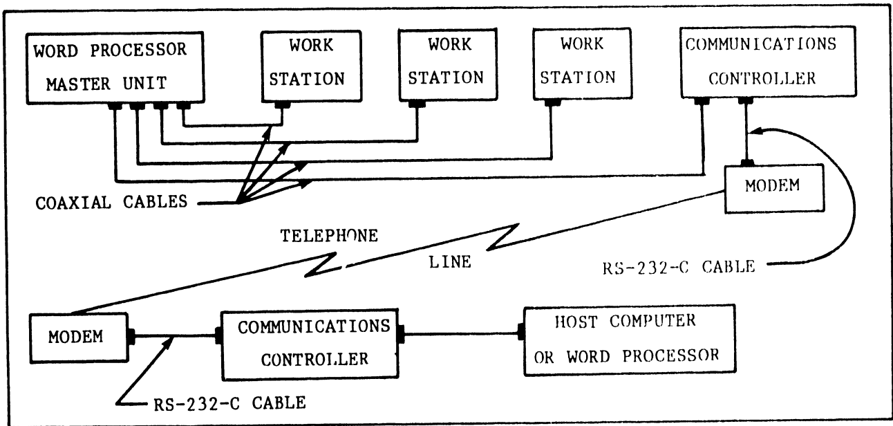
FIGURE 2.3 A TYPICAL BISYNCHRONOUS REMOTE CONNECTION
